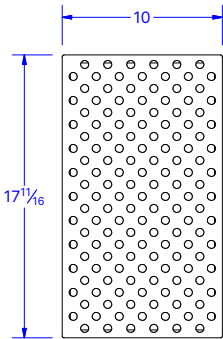
DRYING RACK
